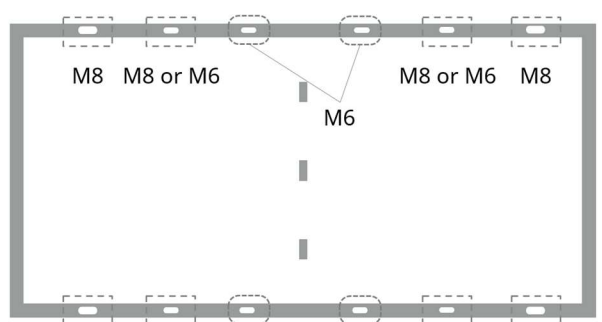
Bolt locations on the module
