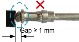
Incorrect crimping
