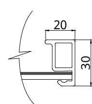
Frame Cross Section
