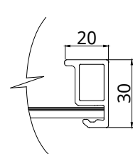
Frame Cross Section
